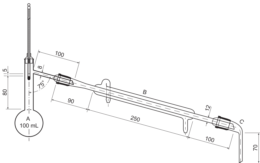
Figure 2.2.11-1. – Apparatus for the determination of distillation range
